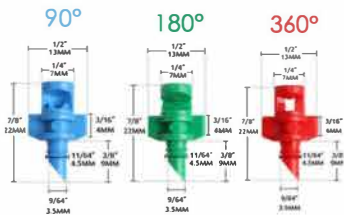
ONE WAY FOGGER 8mm THREADER
